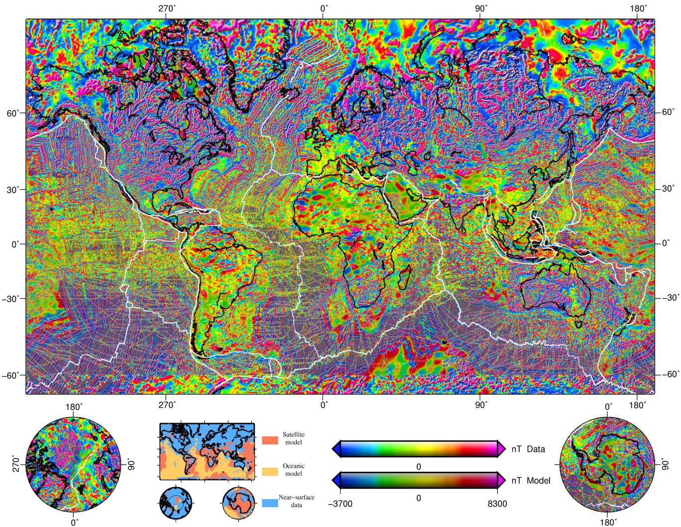
Image: Korhonen, J.V., Fairhead, J.D., Hamoudi, M., Hemant, K., Lesur, V., Mande, M., Maus, S., Purucker, M., Ravat, D., Sazonova, T., and Thebaud, E., 2007, Magnetic Anomaly Map of the World (and associated DVD), Scale: 1:50,000,000, 1st edition, Commission for the Geological Map of the World, Paris, France.
